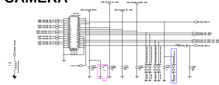
MAIN_CAMERA (16M)
